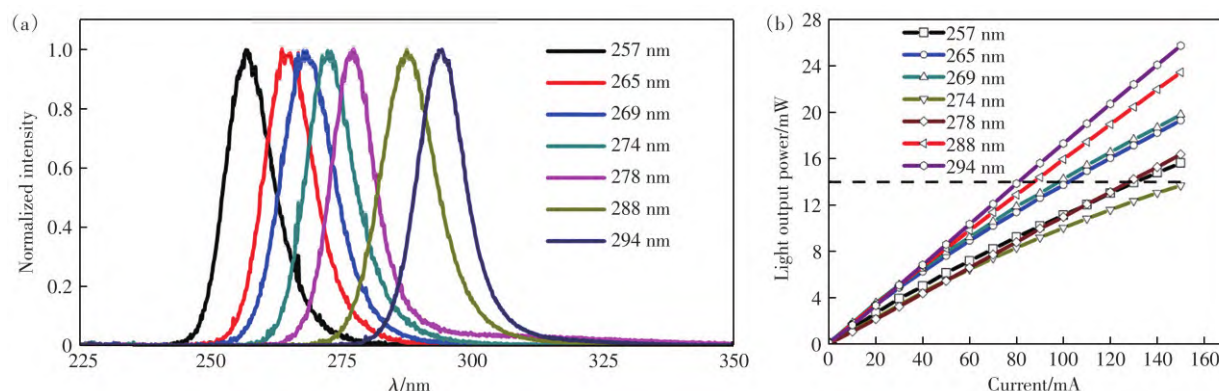
图 3 (a)不同中心发光波长 AlGaIn 基 LED 的 EL 测试发光光谱归一化强度;(b)不同工作电流下 LED 的光输出功率 Fig.3 (a) Normalized EL luminescence spectra of AlGaIn based LEDs with different central emission wavelengths. (b) Light output power of LEDs under different operating currents
