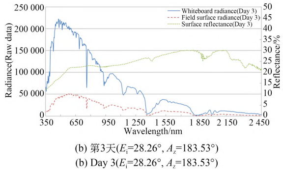
图 11 标准白板法场地实测反射率曲线 Fig. 11 Measured reflectance of field by whiteboard method
