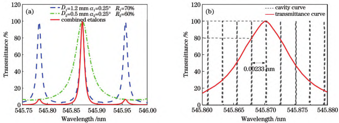
图 6 F-P 标准具的透过率。(a) 0.25 nm 范围内两 F-P 标准具组的透过率;(b) 0.02 nm 范围内两 F-P 标准具组的透过率 Fig. 6 Transmittance of F-P etalon. (a) Combined transmittance of two F-P etalons in the range of 0.25 nm; (b) combined transmittance of two F-P etalons in the range of 0.02 nm
