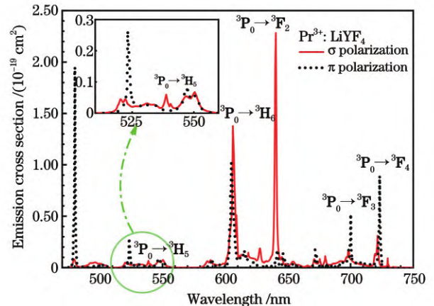
图 3 \text{Pr}^{3+}:\text{LiYF}_4 晶体的偏振发射截面 Fig. 3 Polarization-dependent emission cross section of a \text{Pr}^{3+}:\text{LiYF}_4 crystal (the inset shows the details of the investigated emission spectrum)
