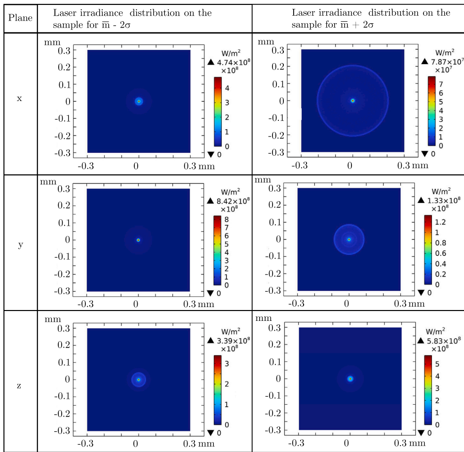
Fig. 13. Comparison of the simulated irradiance distributions for concept 1 at the focus point on the sample considering the maximum and minimum 2\sigma deviations regarding the points T_1 - T_4 .
