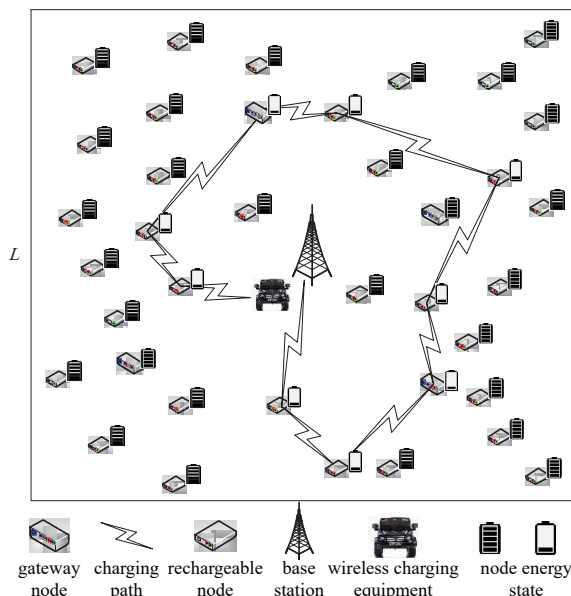
Fig.2 WRSN network model
