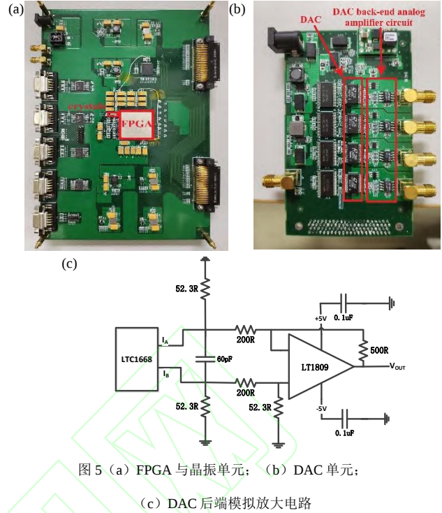
Fig.5 (a) FPGA and crystal oscillator unit; (b) DAC unit;
