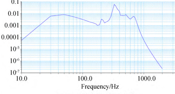
(c) Z方向随机振动响应曲线 (c) Z-random vibration response curve
