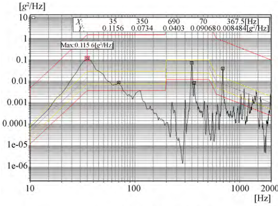
(c) Z方向随机振动响应曲线 (c) Curve of Z-random vibration response
