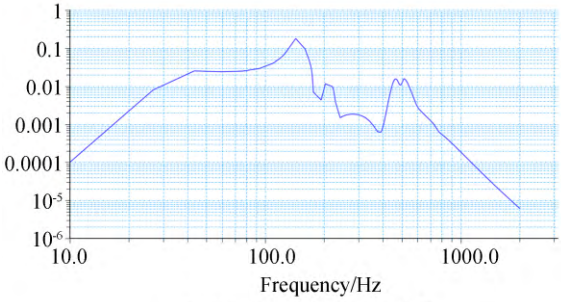
(b) Y方向随机振动响应曲线 (b) Y-random vibration response curve
