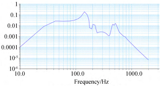
(a) X方向随机振动响应曲线 (a) X-random vibration response curve
