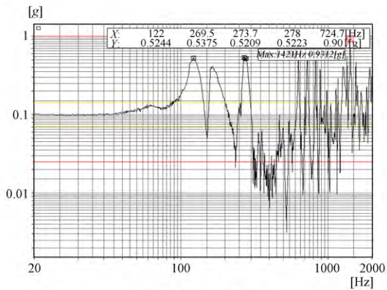
(b) 安装金属橡胶减振器 (b) Installed with metal rubber vibration absorber
