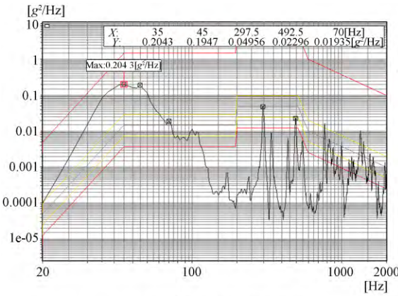
(b) Y方向随机振动响应曲线 (b) Curve of Y-random vibration response
