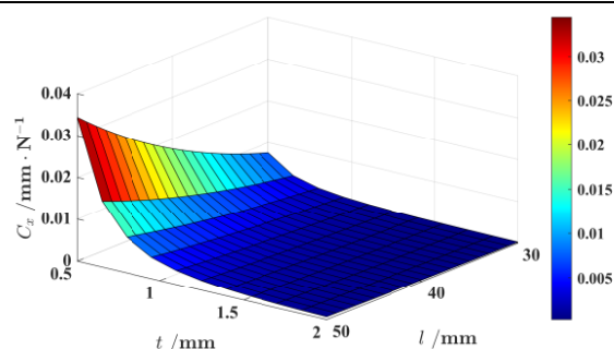
(c) 柔性度 C_x 随设计参数 t 和 l 的变化关系 (c) The relationship between flexibility C_x and design parameters t and l
