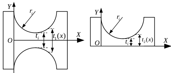
(a) 圆弧形柔性铰链
