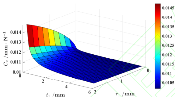
(a) 柔性度 C_x 随设计参数 t_1 和 r_1 的变化关系; (a) The relationship between flexibility C_x and design parameters t_1 and r_1
