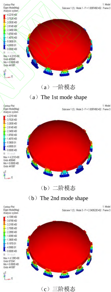
(c) The 3rd mode shape
