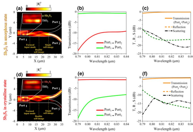
Fig. 4. Simulated device performance for a-Sb 2 S 3 (upper panel) and c-Sb 2 S 3 (lower panel). (a) and (d) Full-wave simulation showing the optical field intensity |E|^2 in the switch for the fundamental TE mode in the xy plane at \lambda = 800 nm. The boundaries of the SiN waveguide and metasurface structure are indicated by dashed lines and rectangles, respectively. Inset: enlarged view of the field profile in the metasurface. (b) and (e) Transmission spectra at two output ports Port 2 and Port 3 . (c) and (f) Total transmission at output ports (Port 2 + Port 3 ), reflection, and scattering of the device.
