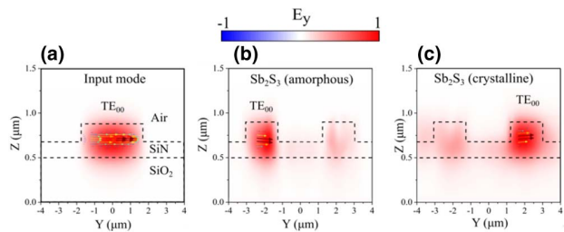
Fig. 12. Modes in the input and output ports of SiN waveguides. Simulated E_y component at \lambda = 800 nm for the \text{TE}_{00} mode in the (a) input stem SiN waveguide before interacting with the metasurface, (b) output Port 3 for a - \text{Sb}_2\text{S}_3 and (c) output Port 2 for c - \text{Sb}_2\text{S}_3 . The arrows indicate the vector diagrams of the electric field component of the modes. The dashed black lines show the boundaries of the SiN waveguides.
