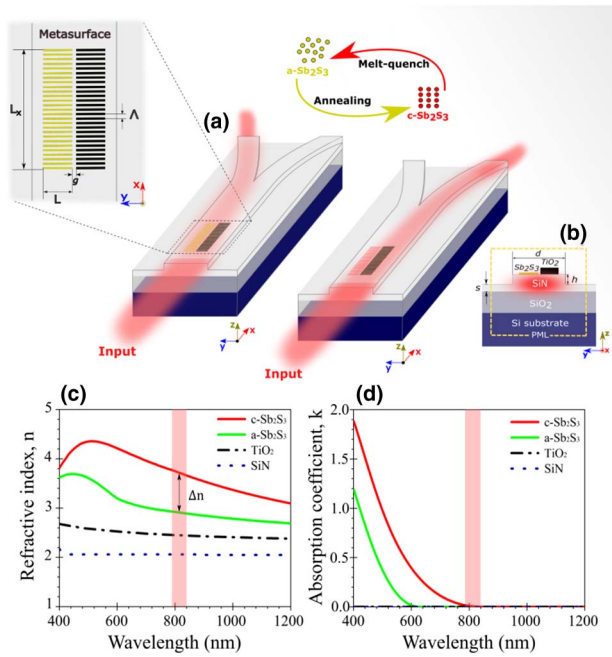
Fig. 1. Design of the proposed metasurface-based reconfigurable (1 \times 2) integrated switch working around \lambda = 800 nm. (a) 3D illustrations of the device structure and its functionality when the \text{Sb}_2\text{S}_3 metasurface structure is in a crystalline or amorphous state. The top-left inset shows the top view of the device with dimensions of the metasurface consisting of a set of passive \text{TiO}_2 nanorods and another set of PCM ( \text{Sb}_2\text{S}_3 ) nanorods. The top middle inset shows the conditions required for the \text{Sb}_2\text{S}_3 to undergo a reversible structural transition from amorphous to crystalline states. (b) Cross section of the device. (c) and (d) Wavelength dependence of the complex optical constants ( n , k ) of amorphous \text{Sb}_2\text{S}_3 , crystalline \text{Sb}_2\text{S}_3 , amorphous titanium dioxide, and silicon nitride. Highlighted parts in red indicate the spectral region of interest where \text{Sb}_2\text{S}_3 exhibits low loss and high switching contrast.
