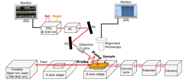
Fig. 10. Schematic illustration of the experimental setup suggested for characterizing the performance of the proposed reconfigurable switch. Here, PPG is a programmable pulse generator, PC is a power controller, and M is a mirror.
