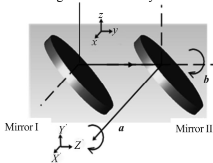
Fig.4 The relative motion of the two mirrors
