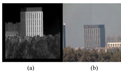
Fig.11 Images of multiband co-aperture optical system: (a) Infrared image; (b) Visible image
