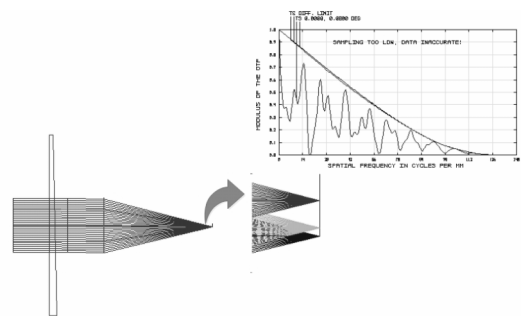
Fig.9 Parallel plate set in parallel optical path
