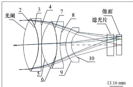
图 1 紫外光学系统结构图 Fig.1 Structure of ultraviolet optical system
