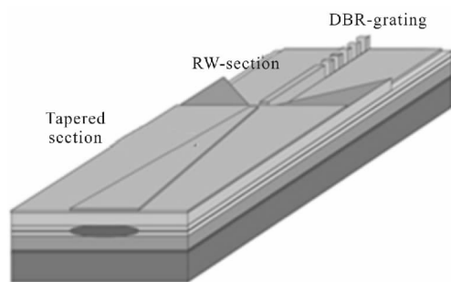
图 3 带有 DBR 光栅的锥形激光器示意图 Fig.3 Typical tapered laser with DBR gratings
