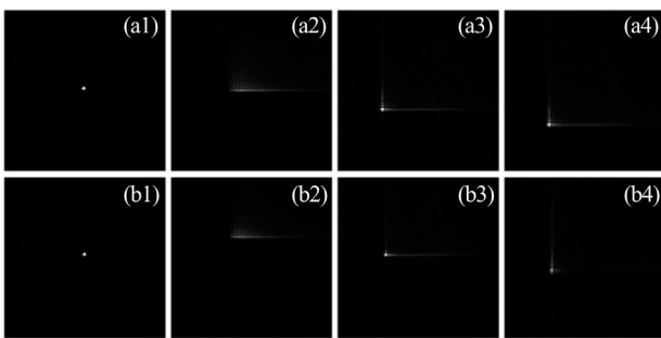
Fig.8 Experimental results of the control propagation trajectory of Airy beam: (a1) and (b1) The intensity patterns of a Fresnel lens with focal length of 150 mm; (a2)—(a4) The intensity patterns when removing the central mask position from origin to left by 1.44 mm; (b2)—(b4) The intensity patterns when removing the central mask position from origin to left by 1.44 mm then to upper by 1.44 mm
