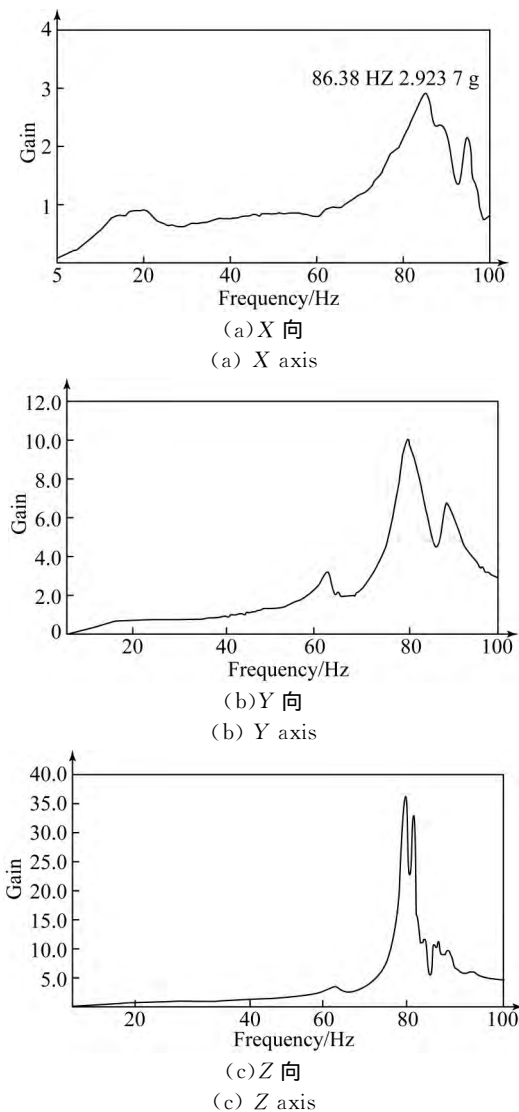
图 15 主镜正弦振动响应曲线 Fig. 15 Frequency response of primary mirror
