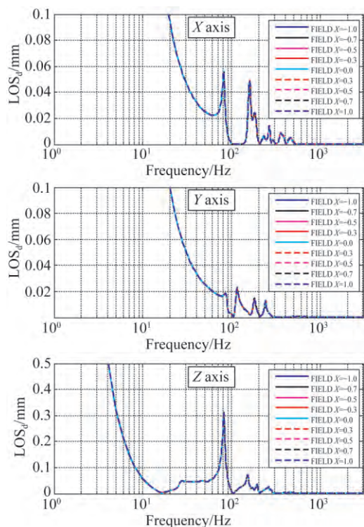
图 13 视轴漂移 LOS_d 的频率响应 Fig. 13 Frequency response of LOS_d
