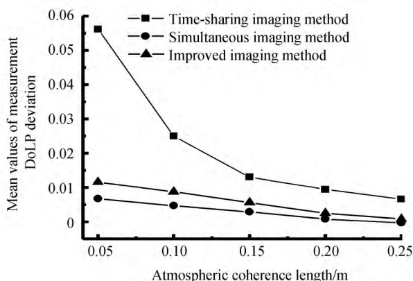
(b) The mean values of measurement DoLP deviation with AO system correction
