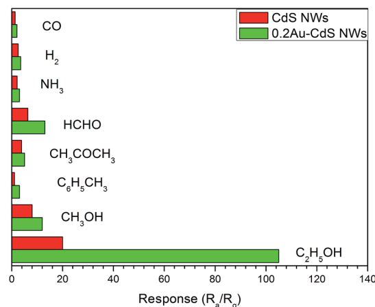
Fig. 8 Selectivity of the sensors to 100 ppm hydrogen ( H_2 ), carbon monoxide (CO), acetone ( CH_3COCH_3 ), ammonia ( NH_3 ), formaldehyde (HCHO), toluene ( C_6H_5CH_3 ), methanol ( CH_3OH ), ethanol ( C_2H_5OH ).
