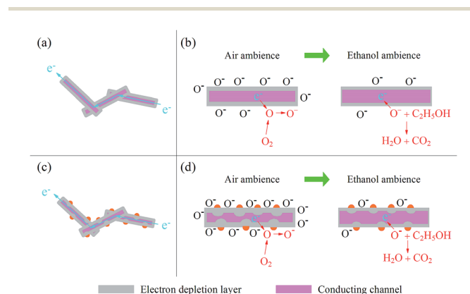
Fig. 9 (a) Electron transmission within and between CdS NW(s), (b) ethanol sensing mechanism of CdS NWs, (c) electron transmission within and between Au–CdS NW(s), and (d) ethanol sensing mechanism of Au–CdS NWs.
