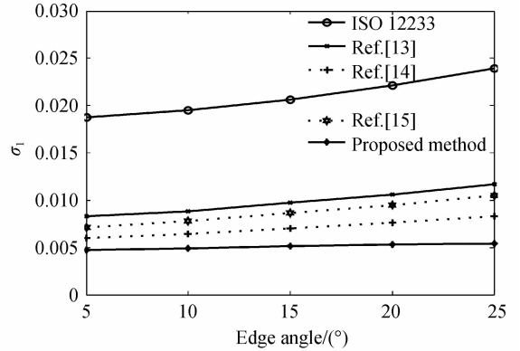
图 4 SNR 为 40dB 时 MTF 测量准确度随刃边倾角的变化 Fig. 4 The results of measurement accuracy of MTF with the change of edge angles at the SNR of 40 dB
