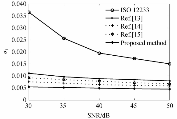
图 5 刃边倾角为 10° 时 MTF 测量准确度随噪声的变化 Fig. 5 The results of measurement accuracy of MTF with the change of SNRs at edge angle of 10°
