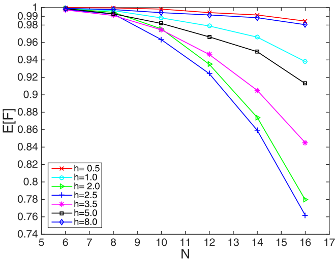
FIG. 3. Averaged fidelity E[F] as a function of system size N for different values of disorder strength h from small to large. The value of h is indicated in the legend. E[F] decays as the system size increases, it decays the fastest when h = 2.5 .
