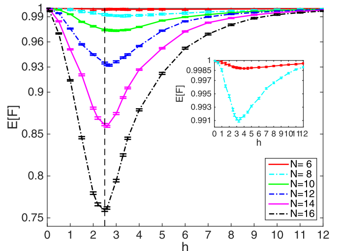
FIG. 1. Averaged fidelity of the dephased state as a function of h for system size from 6 to 16. The system size N is indicated in the legend. Statistical error bars for every data points are given. In the ergodic phase [7] (small h ) E[F] decays substantially under the dynamics until h approaches to the critical point h_c , then in the localized phase (large h ) E[F] turns to increase approximately approaching to 1. The drop gets sharper as system size N increases. The inset corresponds to enlarged pictures for system size N = 6 and 8 with the same data.
