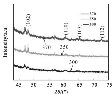
Fig.2 X-ray diffraction scans from 1 500 cycles AlN films grown at 300 °C, 350 °C and 370 °C
