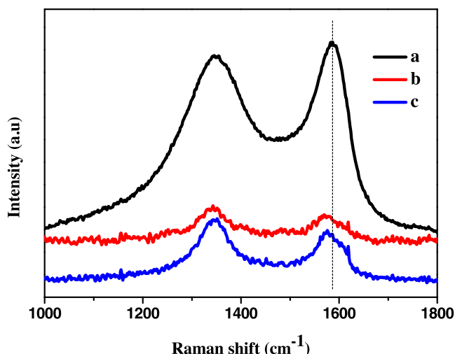
Fig. 5. Raman spectra of GO (a), CdSe/rGO (b), Ca 2+ @CdSe/rGO (c).
