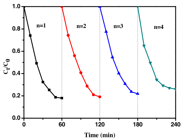
Fig. 12. Repeated experiments of photocatalytic degradation of tetracycline hydrochloride by the prepared \text{Ca}^{2+}@ \text{CdSe}/\text{rGO} sample composite with 6 mol% \text{Ca}^{2+} and 5% GO addition.
