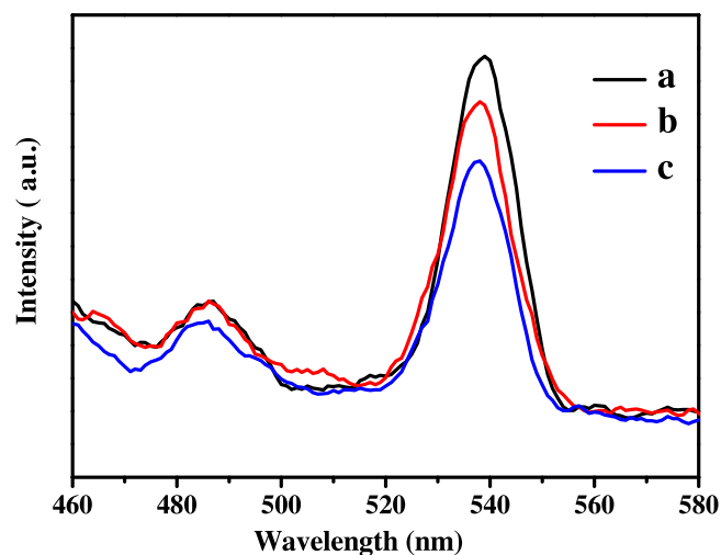
Fig. 7. PL spectra of QDs CdSe (a), CdSe/rGO (b) and Ca 2+ @CdSe/rGO (c).
