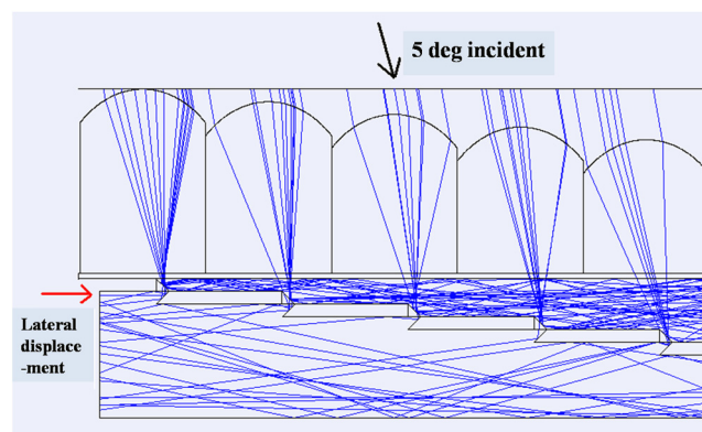
Fig. 7 Lateral displacement tracking with 5 deg of parallel light incidence in elevation.
