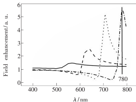
Fig. 3 The field enhancement factor P(\lambda) of Au NP when the dielectric constants of the surrounding medium is 2.2 (solid), 5.2 (dash), 8.2 (dot) and 10.9 (dash dot).
