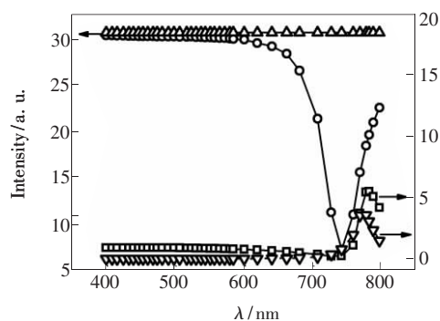
Fig. 2 The electromagnetic-field enhancement factor P(\lambda) ( \square ), nonradiative energy transfer rate \gamma_{\text{et}}(\lambda)/\gamma_{\text{rad}}^0(\lambda) ( \nabla ), and the TPEF enhancement factor A(\lambda) with ( \circ ) and without ( \triangle ) nonradiative energy transfer effect taking into account. The dielectric constants of surrounding medium \varepsilon_0 = 10.9 .
