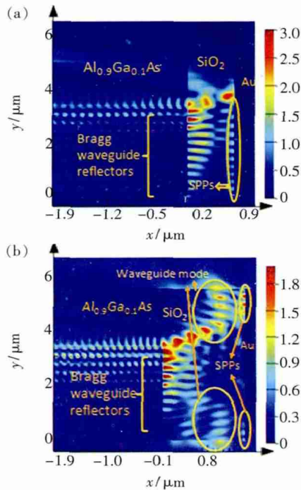
Fig. 9 The electrical intensity along x - y facet intersection at z=0 . (a) \text{SiO}_2 thickness of 700 nm. (b) \text{SiO}_2 thickness of 1500 nm.
