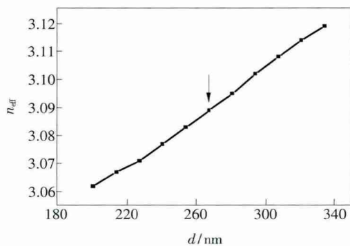
Fig. 3 Relationship between d and mode effective index. For designed effective index at 3.088, the thickness of d is selected at 267 nm.
