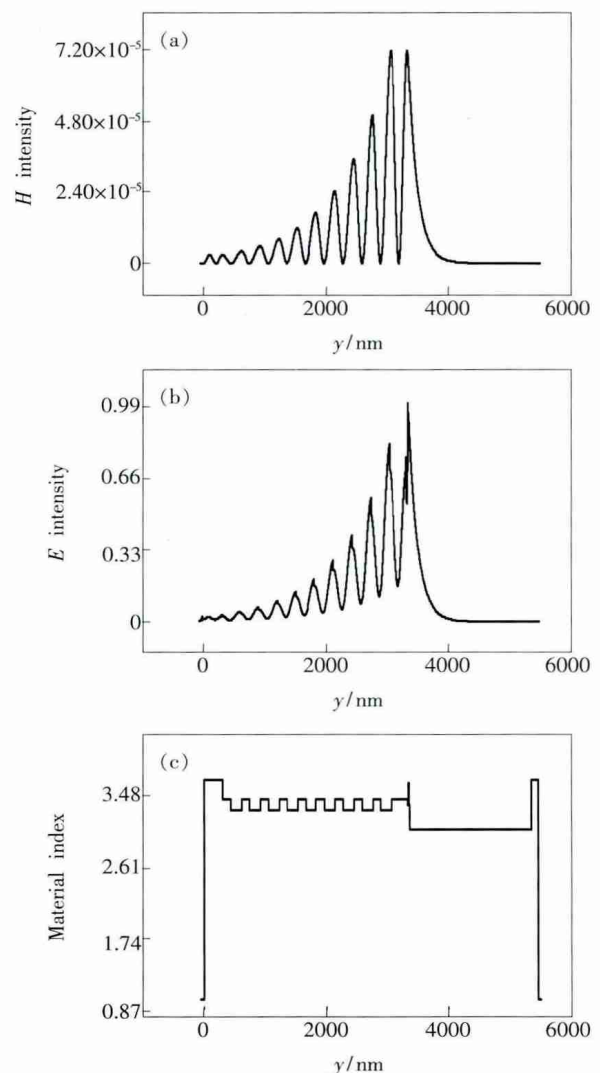
Fig. 5 Optical mode in the designed semiconductor cavity. (a) H intensity of the optical mode along the y axis. (b) E intensity of the optical mode along y axis. (c) Refractive index in the semiconductor part along y axis.
