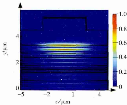
Fig. 6 The calculated optical mode field for TM 00 mode
