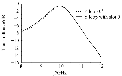
图 6 正入射情况下两种结构透射比对照 Fig. 6 Measured frequency response characters under perpendicular incidence
