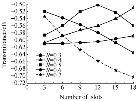
图 4 设置不同圆孔后对应中心频点的透过率 Fig. 4 Transmittance at resonance frequency vs different radii and number of circular slots
