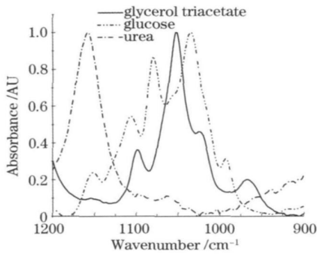
图 2 三乙酸甘油酯、葡萄糖和尿素的归一化光谱 Fig.2 Normalized spectra of glucose, urea and glycerol triacetate
