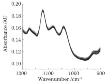
图 4 手指的原始光谱 Fig.4 Raw ATR-FTIR spectra of finger
