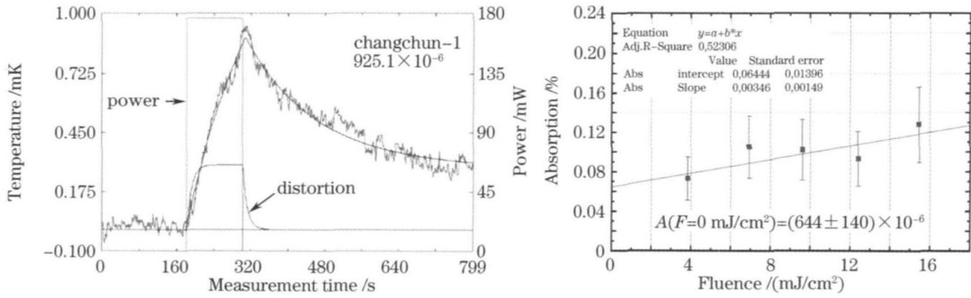
图 2 (a) 193 nm 激光量热吸收测试中样品温度变化曲线; (b) CaF 2 衬底吸收随辐射激光能量密度的变化 Fig. 2 (a) Variation of sample temperature with time obtained by 193 nm laser calorimeter; (b) variation of CaF 2 substrate absorption with laser fluence level
