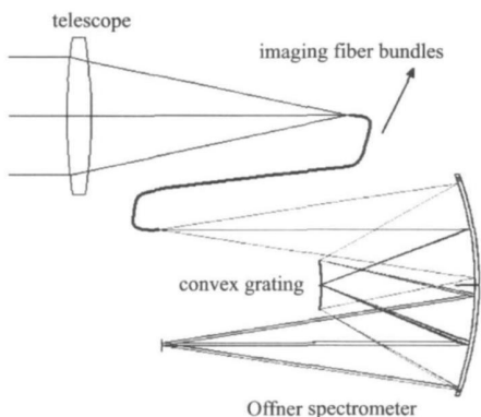
Fig. 1 Structure sketch of imaging fiber-optic spectrometer
