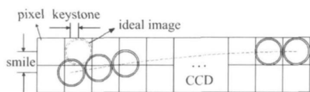
Fig. 2 Scheme of misalignment between image of fiber-optic and CCD pixels
