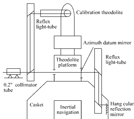
Fig. 1 Heading calibration system and optical path of calibration theodolite
