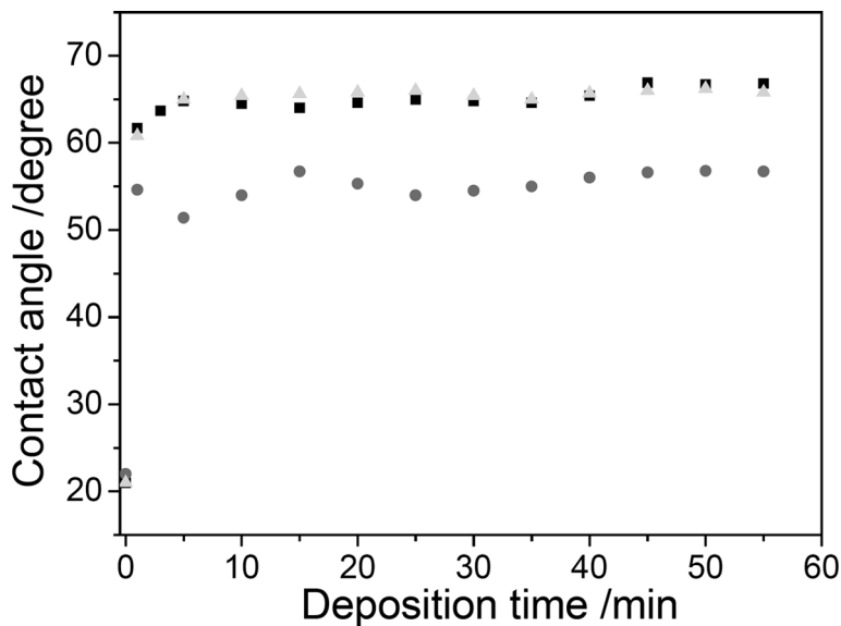
FIGURE 1 Contact angles of self-assembled monolayers as a function of deposition time (▲: film with trifluoromethyl benzene end, ■: film with cyano benzene end, and ●: film with ethylic benzene end).
