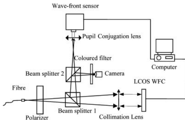
Figure 5. The optical layout of an adaptive optics system.
