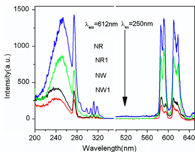
Figure 4. The excitation spectra (left) of \text{GdPO}_4:\text{Eu}^{3+} samples measured at room temperature and monitored at 612 nm (left). The emission spectra (right) of the samples measured at room temperature and excited at a maximum of the CTB band.
