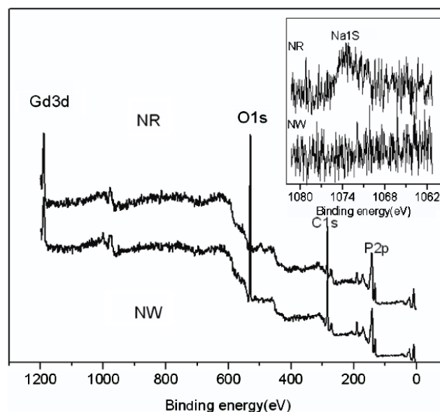
Figure 6. XPS spectra of samples NR and NW.
