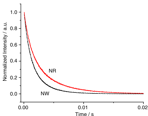
Figure 7. The fluorescence lifetime curves of NR and NW monitored at 612 nm emission of \text{Eu}^{3+} .
