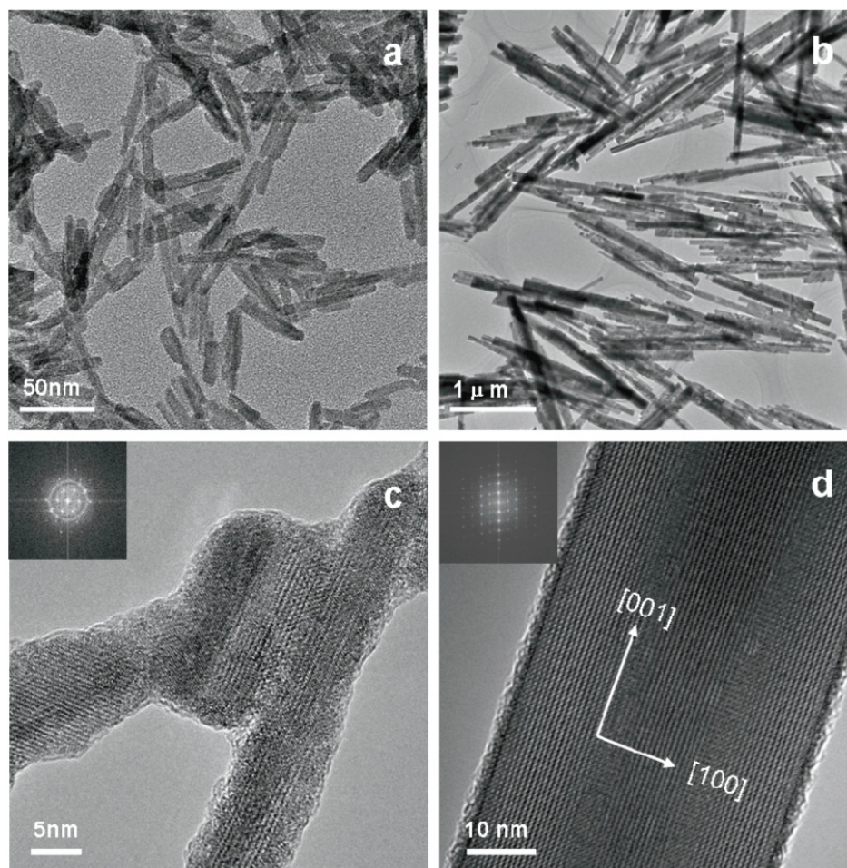
Figure 2. TEM images recorded from as-synthesized samples: (a) and (c) NR; (b) and (d) NW. The insets are the fast Fourier transform diffraction patterns (FFT).
