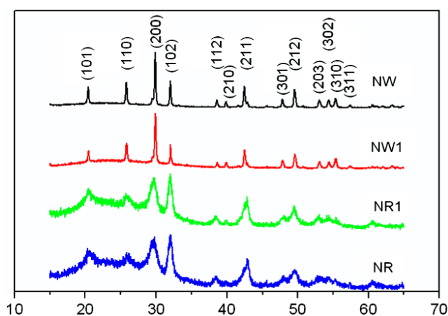
Figure 1. XRD patterns of samples NR (5%-Eu, pH = 10), NR1 (3%-Eu, pH = 10), NW (5%-Eu, pH = 2) and NW1 (3%-Eu, pH = 2).
