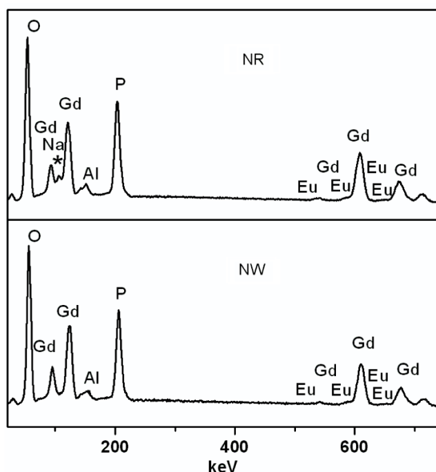
Figure 5. EDS spectra of samples NR and NW.
